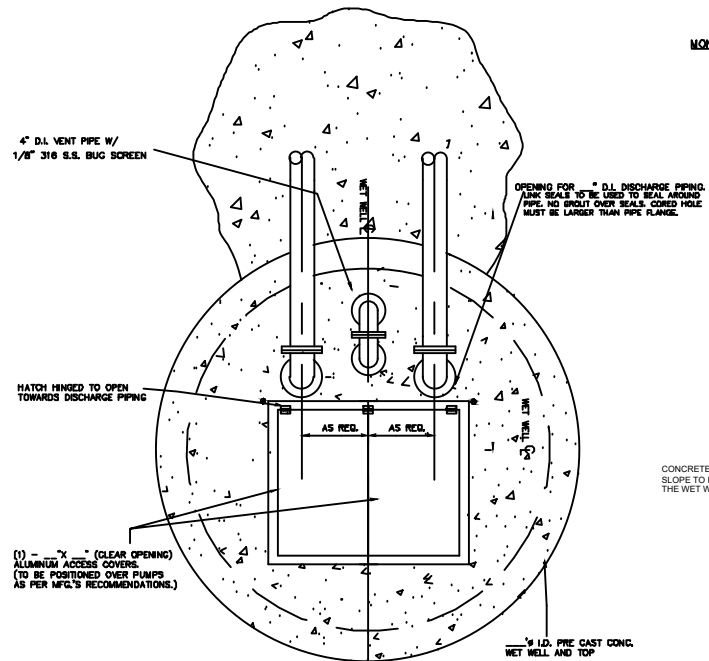
OPENING DETAIL — PLAN VIEW N.T.S.
