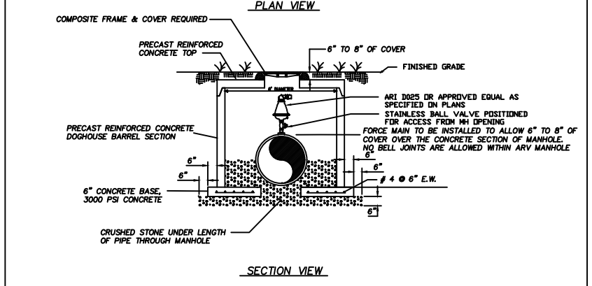
SEWER AIR RELEASE VALVE AND MANHOLE NTS
