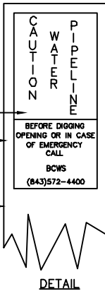
LINE MARKER
