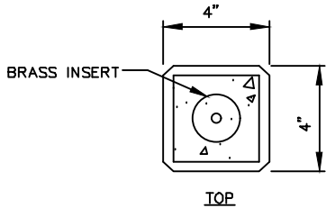
VALVE MARKER
